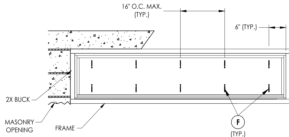
FRAME ANCHORING 2X Buck
